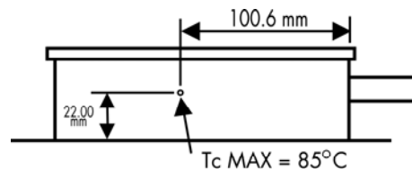
Case Temperature Measurement Location
